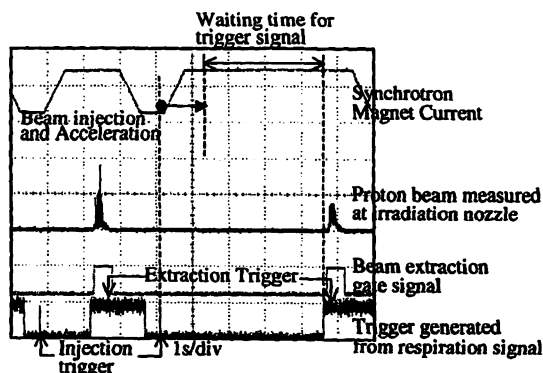
Figure 6 Respiration synchronized operation.
