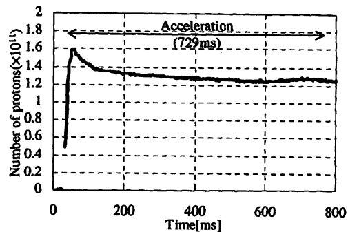
Figure 2: Number of protons accelerated up to 250MeV.
