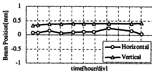
Figure 4 Stability of beam position
