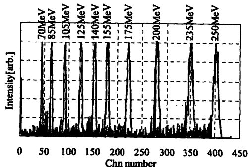
Figure 3: Results of energy measurement by MLC
